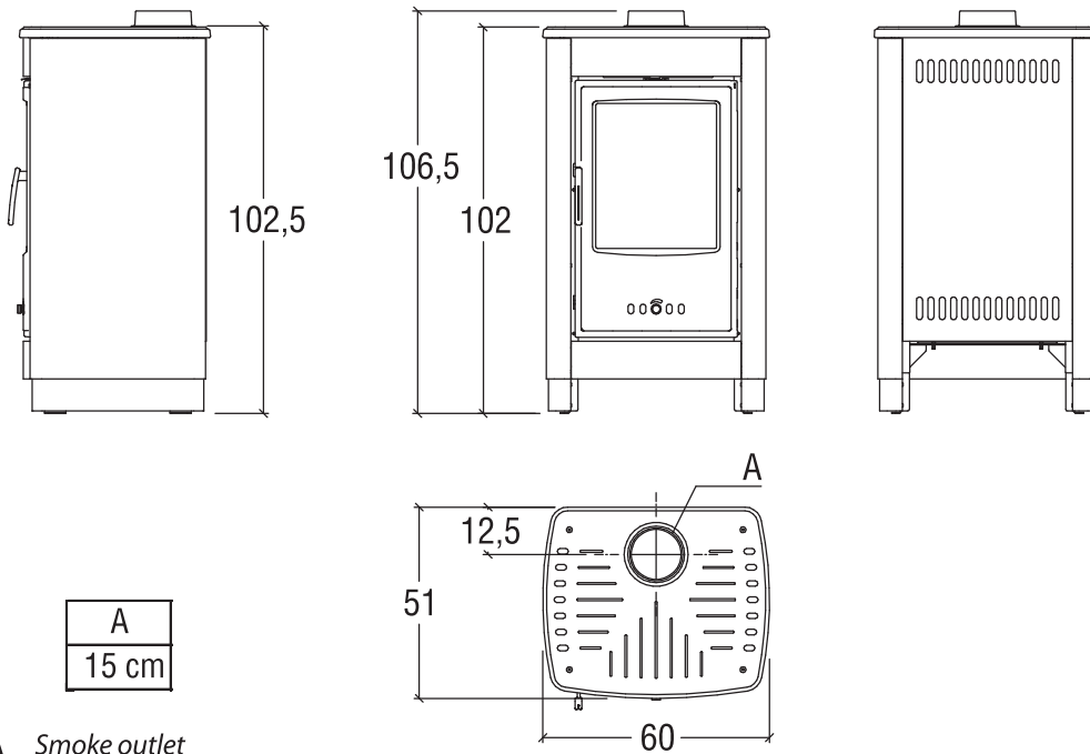
A Smoke outlet
